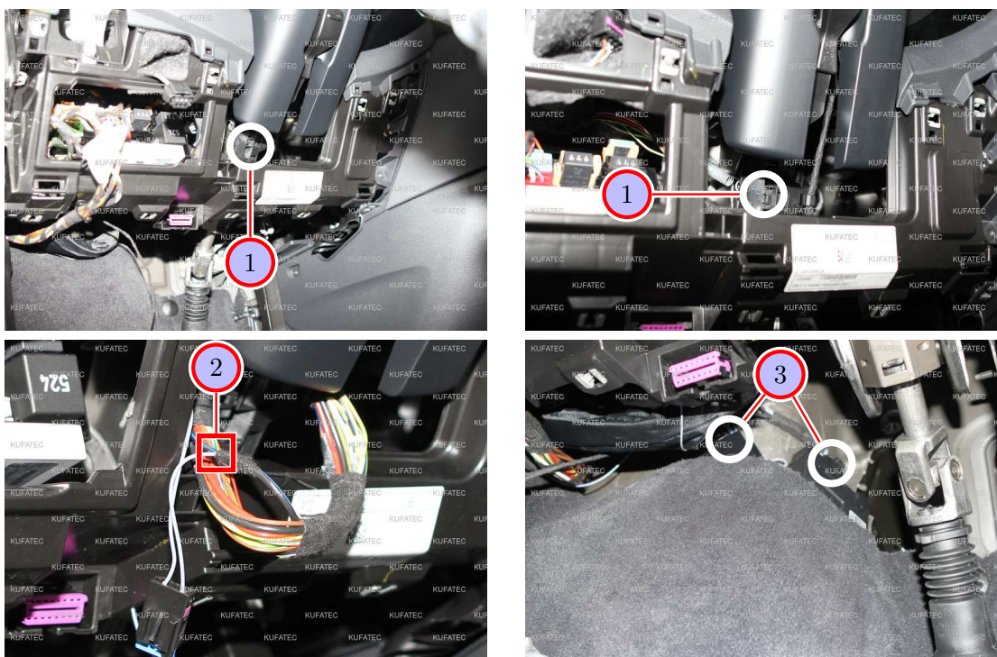
Figure 9: Connection ignition lead / control units
